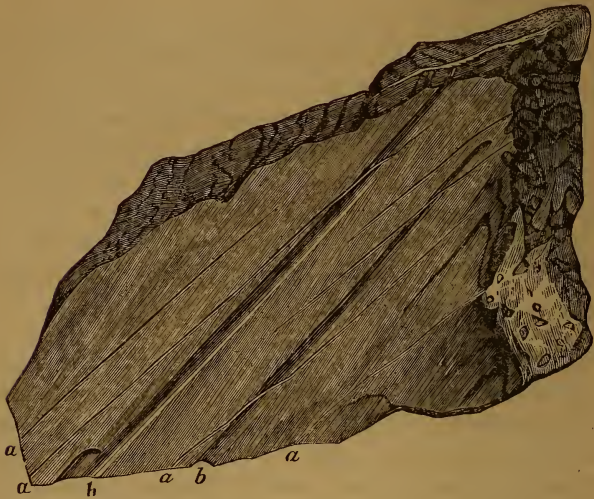
Fig. 3.—Block of Limestone furrowed, scratched, and polished, from the Glacier of Rosenlauri, Switzerland. (Lyell.)
